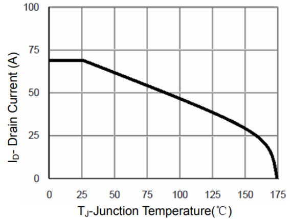
Figure 10 Current De-rating
